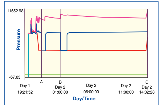
Example Total Plot of Sigrá Drill Stem Test (DST)
